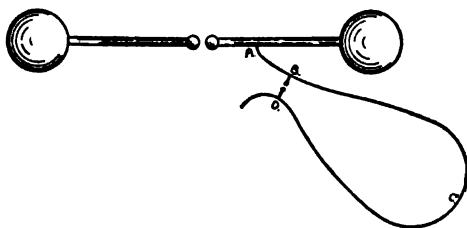
FIG. 30.—A method of investigating wave forms. A current from the oscillator travels along the wire ABCD, a loop of which is bridged by a spark-gap, BD. Owing to the finite velocity of propagation there will be a difference of potential between B and D, of which the spark-length is a measure.
