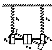
FIG. 125.—The masses M_1 and M_2 of FIGS. 123 and 124 divided, and part of each moved to the middle of the rod. If the ratio M_1:M_2 is equal to M_m:M_2 , the system vibrates about M_m as a fulcrum with an increased frequency.
