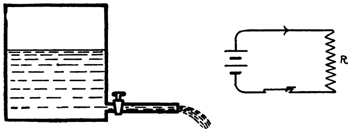
FIG. 9.—Model illustrating the flow of a conduction current in a conductor, R . The flow continues undiminished as long as the pressure is maintained. The energy expended in friction takes the form of heat and is lost.
