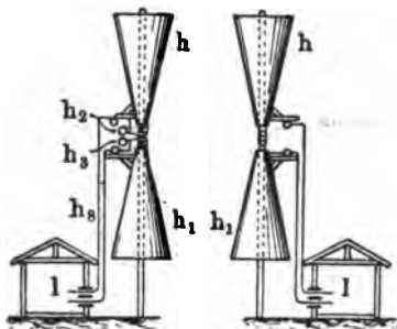
FIG. 71.— Lodge's conical capacity-areas.
