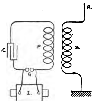
FIG. 78.—Transmitting apparatus with high-frequency transformer. P is the primary of the transformer, whose circuit is closed through the condenser C and spark-gap G; S, the secondary, connected to the antenna A and to ground, and I the induction coil.
