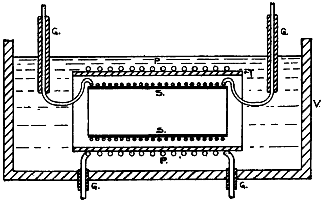
FIG. 77.—A high-frequency transformer, as constructed by Prof. Elihu Thomson. P is the primary winding, S the secondary, and T a glass tube separating the two. V is a vessel of oil in which the coils are immersed, and G G are glass or rubber bushings for further insulating the terminals.
