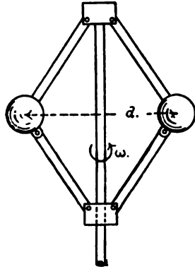
FIG. 6.—Model illustrating the mechanical action of currents. The balls tend to separate, thus increasing their kinetic energy if the angular velocity be kept constant. This energy is supplied from without in overcoming the inertia reaction due to the separation.
