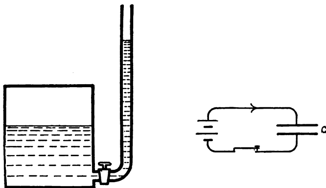
FIG. 8.—Model illustrating the flow of a displacement current in a dielectric C. The pressure in the vessel represents the voltage of the battery; the height of the column, the displacement in the dielectric; the flow of water, the charging current. The energy expended may be recovered.
