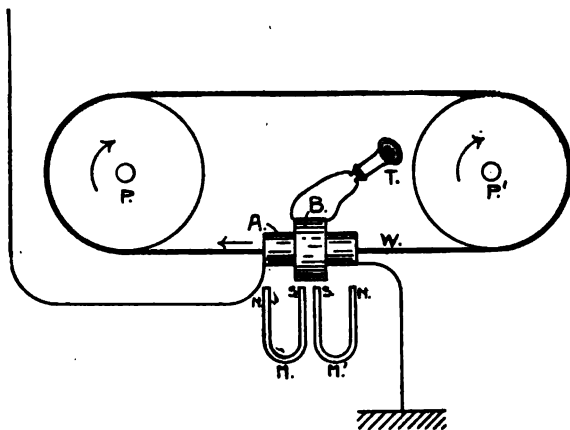
FIG. 103.—Marconi's magnetic detector — Improved form. W is a continuous band of iron wires, passing over the pulleys P P', and threading the coils A and B. M and M' are fixed permanent magnets.
