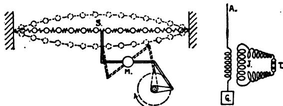
FIG. 137.—Model illustrating the operation of Marconi's "jigger," whose distributed capacity and inductance (elasticity and mass) are so proportioned to the frequency that the current (velocity) imparted through the mutual induction (mass M ) to the secondary (weighted spring) is transformed into potential (tension) at the free terminals of the coil (ends of spring).
