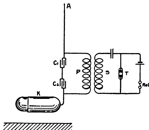
FIG. 140.—Braun system—receiver. The primary resonant circuit C_1C_2P is coupled “elastically” to the antenna through the agency of the condensers C_1 , C_2 , and inductively to the coherer circuit through the transformer P , S .
