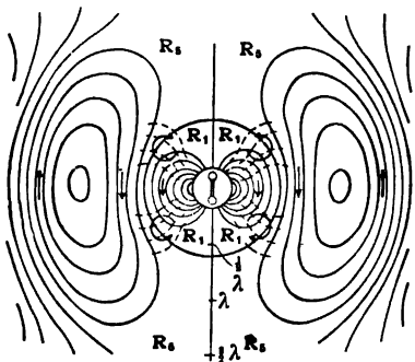
FIG. 90.—The field about the oscillator after an eighth period ( t = \frac{1}{8} T ). The conductors are becoming charged and Faraday tubes are spreading out from them, filling the region within the circle R_1 .
