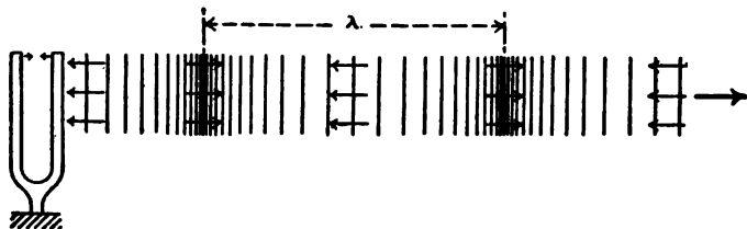
FIG. 12.—Mode of propagation of a longitudinal vibration, such as a sound wave. The crowding and separating of the parallel lines represent condensations and rarifications of the air, and the arrows indicate the motion of individual particles.
