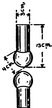
FIG. 26.—Hertz's small oscillator, consisting in two short brass rods terminating in spheres at the inner ends.
