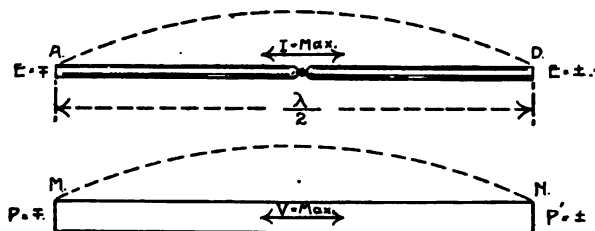
FIG. 23.—An open resonator, AD, compared to a sonorous tube, MN, closed at both ends. The current, which is analogous to the velocity of the air, is a maximum in the middle, but is zero at the ends, as indicated by the dotted curves. The wave-length, \lambda , is twice the length of the resonator.
