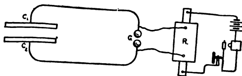
FIG. 20.—An electrical oscillator, consisting in two conductors C_1 , C_2 , joined by a wire interrupted by a spark-gap G . The conductors are charged by an induction coil R , and discharged across the air-gap.
