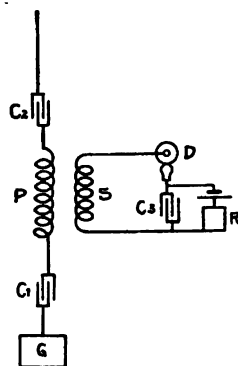
FIG. 142.—Lodge-Muirhead system—receiver. Condensers C_1 and C_2 in series with the antenna and primary P of transformer. Mercury-steel coherer D, in secondary circuit, operating syphon recorder R.
