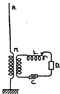
FIG. 129.—Receiver with closed circuit detector D in a local resonant circuit. DCMIL. The inductance L is made variable for the purpose of tuning.
