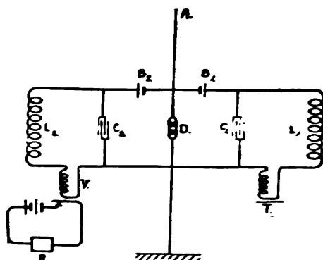
FIG. 145 — Blondel's method of electrical tuning to group frequencies, showing two receivers. The local circuits C_1L_1T_1 and C_2L_2V_2 , with capacities C_1 , C_2 and inductances L_1 , L_2 , are tuned to their respective spark frequencies. On the right is shown a mono-telephone T_1 for receiving by ear, and on the left a vibrating relay V_2 with recording apparatus R .
