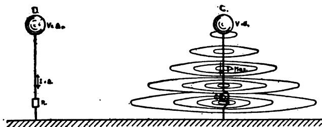
FIG. 66.— Signalling by electromagnetic waves. The conductor C (cf. FIG. 61) is charged by a source G of high-frequency alternating current, and excites waves which expand until they reach the receiving conductor D, and induce alternating currents which are detected by the receiving apparatus R. The circles indicate the lines of magnetic force at the moment when the conductor C is discharged, the potential V = 0 , and the current I is a maximum. FIG. 61 shows the electrostatic lines when I = 0 and V = \text{Max.}
