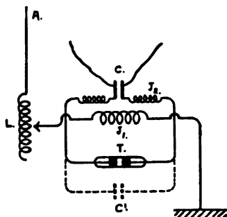
FIG. 131.—Marconi coherer system — receiver. A is the antenna, with variable inductance L, J, J, the zigger, T the coherer and C a condenser, to which the relay and recording apparatus are connected. C' is an additional condenser sometimes used to improve the resonance.
