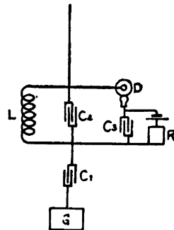
FIG. 143.—Another form of Lodge-Multhead receiver. Inductance L , capacity C_2 , and coherer circuit C_2D , all in multiple.
