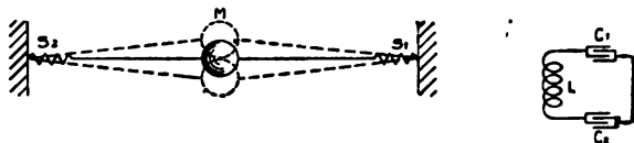
FIG. 136.—Model illustrating the action of an oscillating circuit with concentrated inductance L and capacity C_1, C_2 , which are analogous to the mass M , and the elasticity concentrated in the springs S_1, S_2 .
