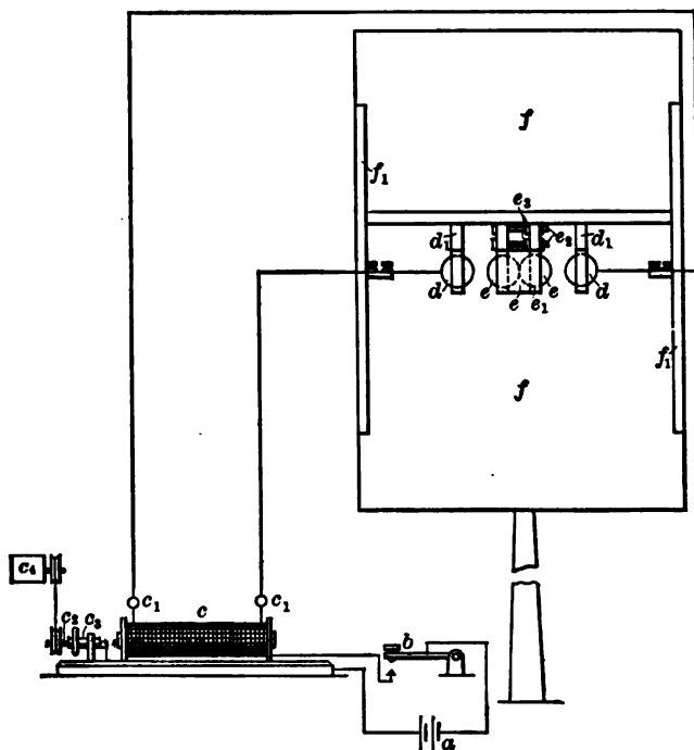
FIG. 68.—Marconi's early transmitting apparatus, consisting in a Righi oscillator, deed , mounted in the focus of a parabolic reflector, f . b is a key for operating the induction coil c .
