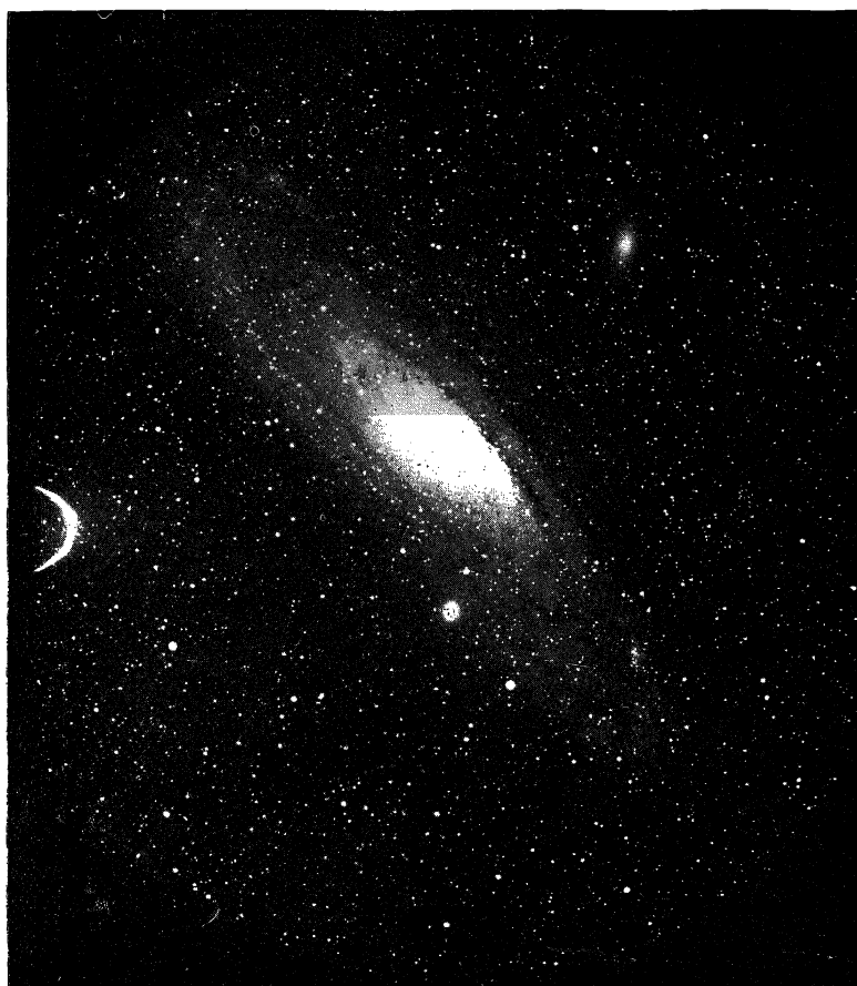
FIGURE 3. THE GREAT ANDROMEDA NEBULA.
